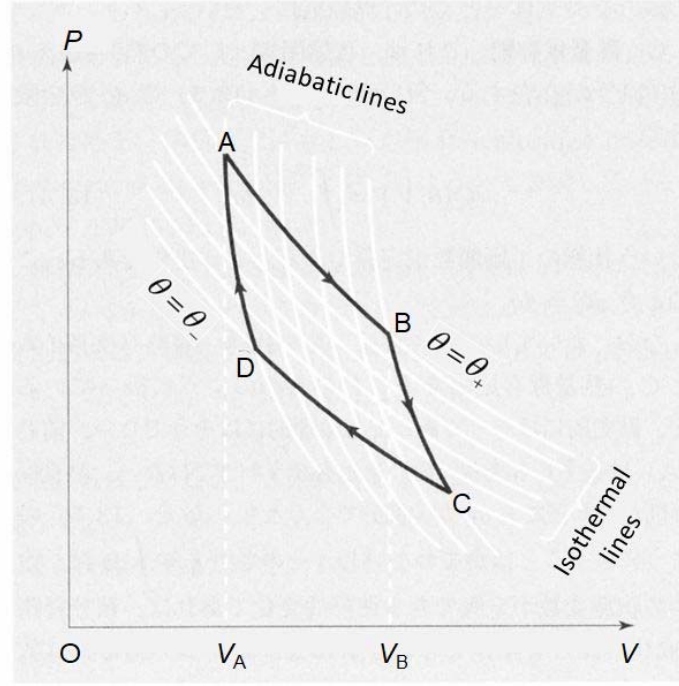
Fig. 20.1 Carnot cycle for ideal gas.
