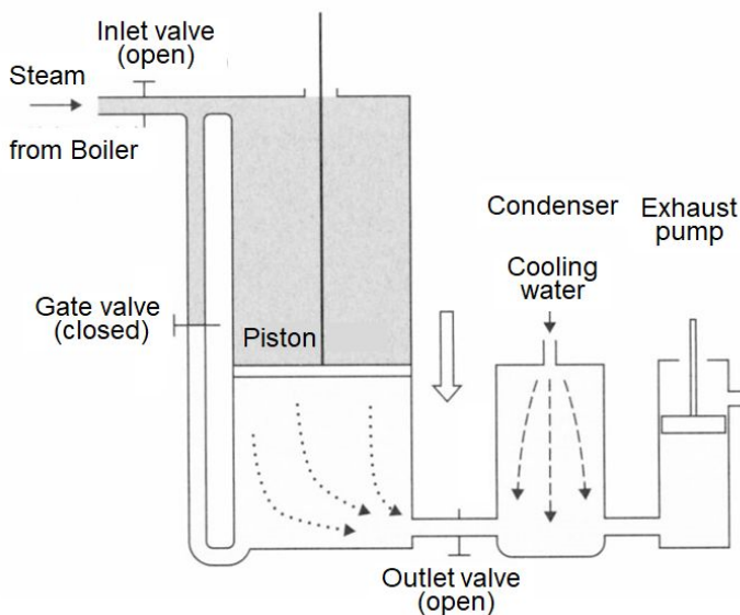
Fig. 18.6 Single-acting steam engine developed by James Watt.
