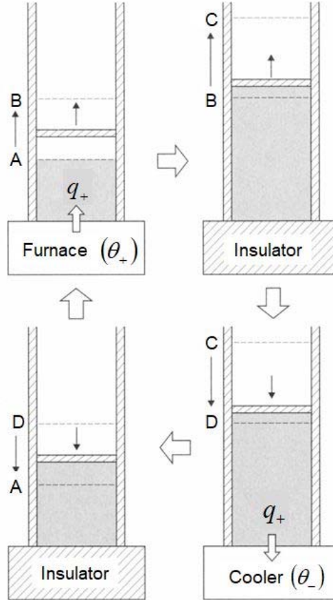
Fig. 19.2 Carnot cycle.
