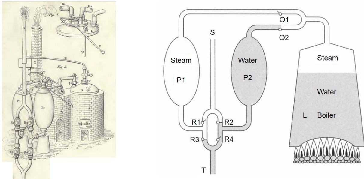
Fig. 18.3 Thomas Savery's steam engine
